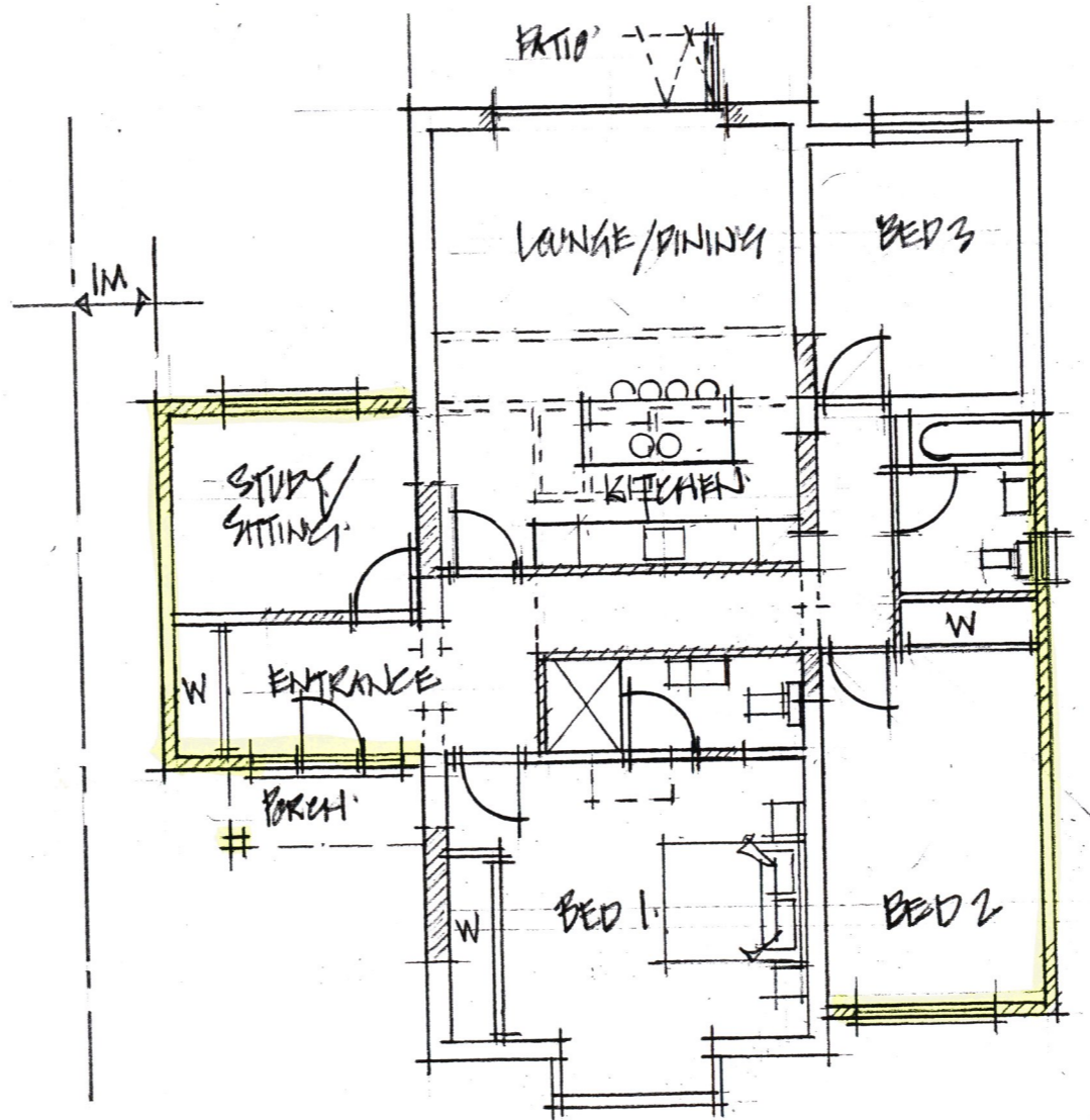
PROPOSED PLAN 1:100
