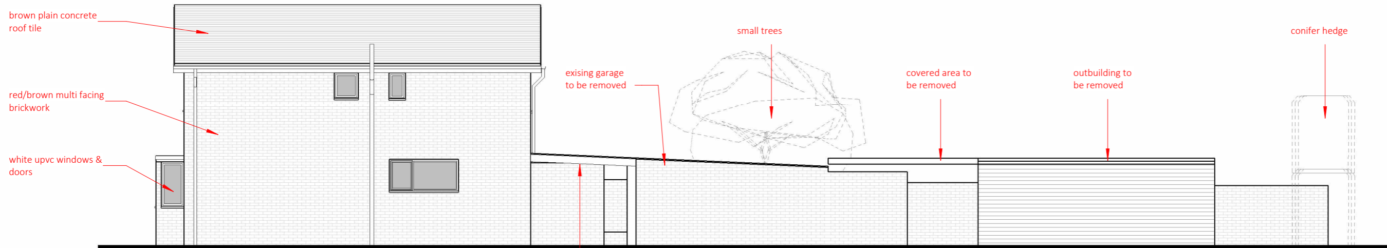
2 P03 north west elevation - existing 1:100
