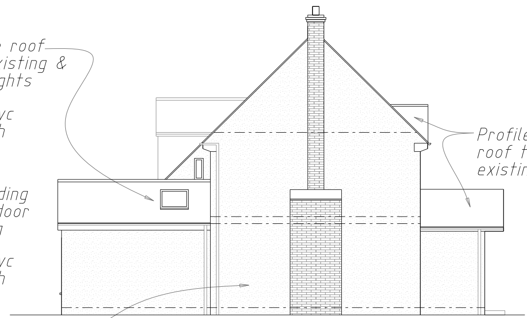
PROPOSED SIDE ELEVATION (E)
