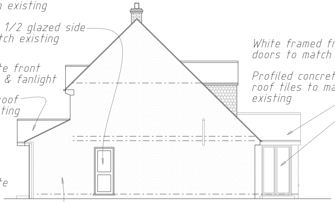
PROPOSED SIDE ELEVATION (W)
