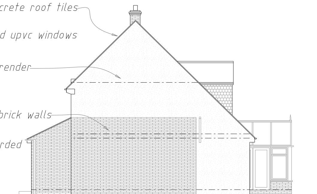
EXISTING SIDE ELEVATION (W)
