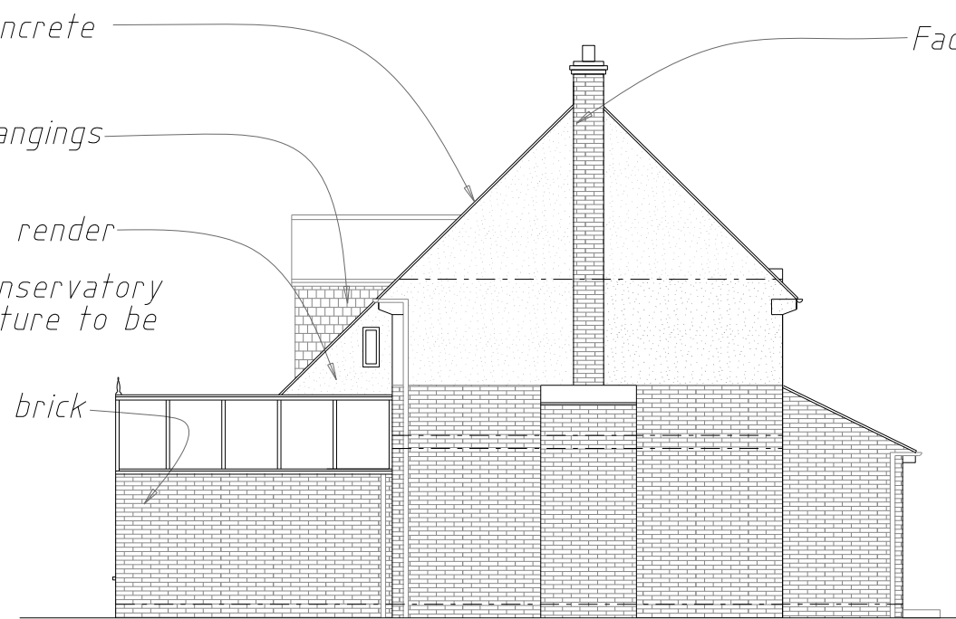
EXISTING SIDE ELEVATION (W)
