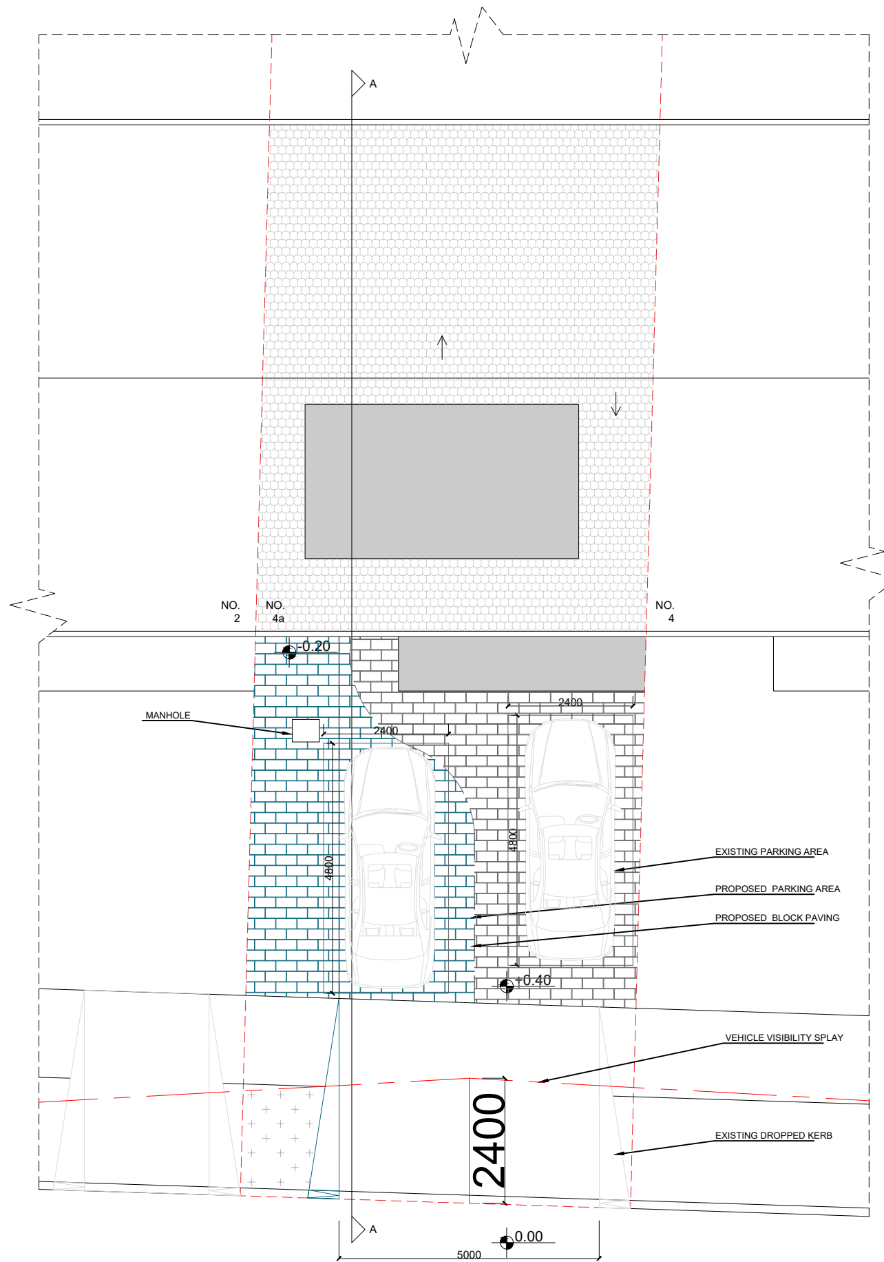
Proposed Visibility Splay Plan
