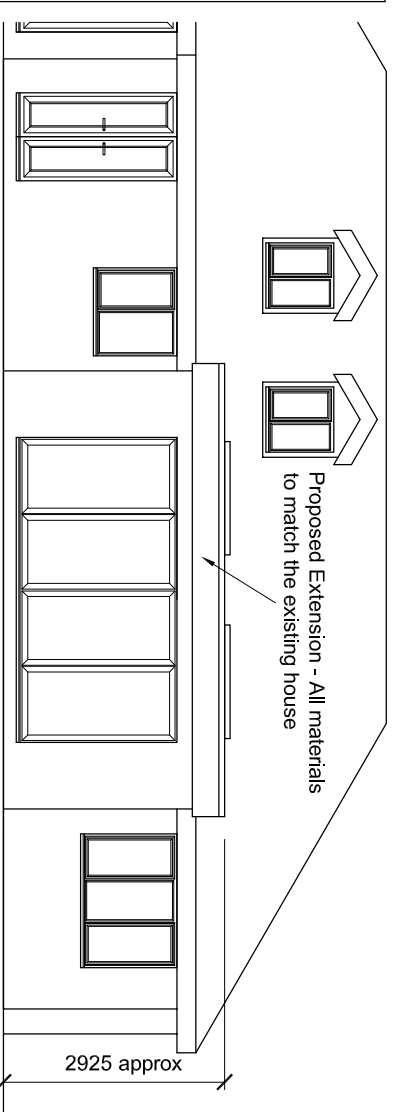
PROPOSED REAR ELEVATION (scale 1:100)
