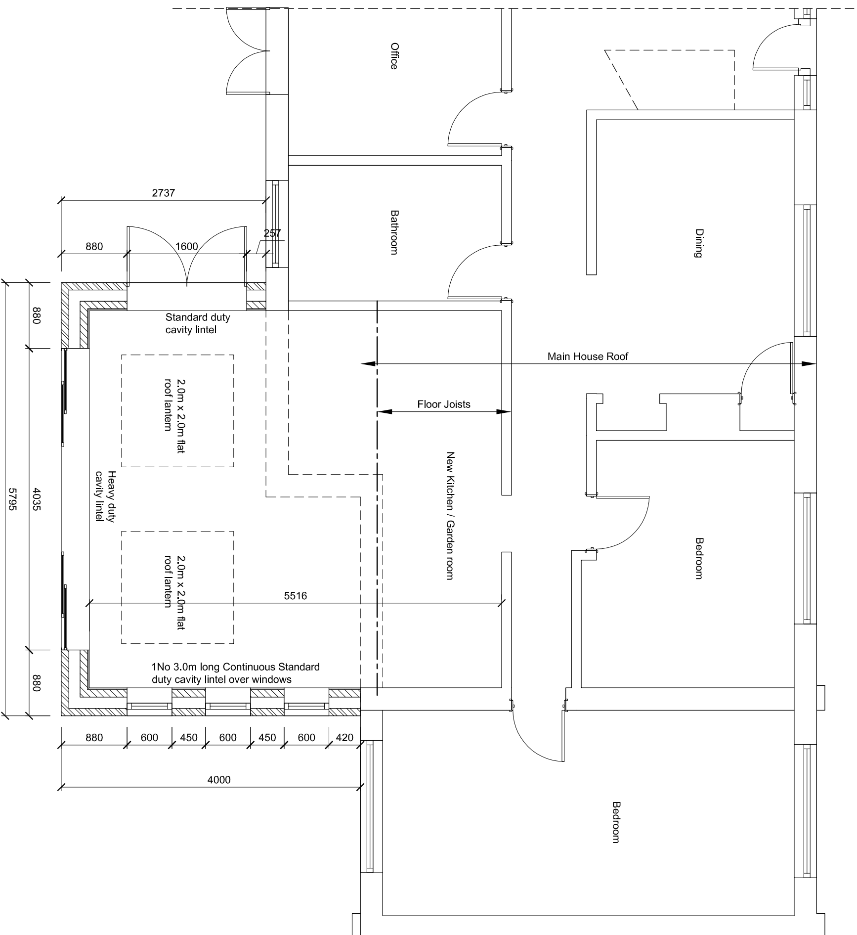
PROPOSED GROUND FLOOR LAYOUT (scale 1:50)
