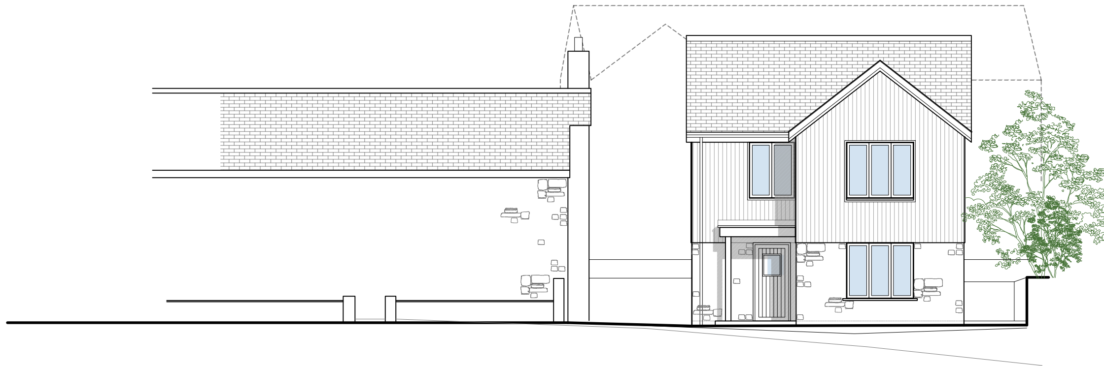
Front Elevation - showing relationship with Bryher Cottage
