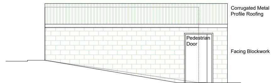
Side (South East) Elevation
