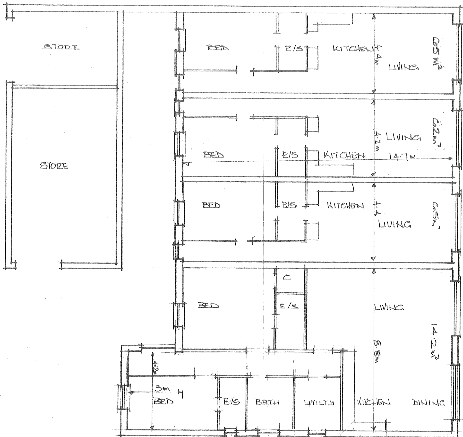
SPARKS BARNs PLAN AS PROPOSED UNITS 1-4. NGA SB5 1:100 @ A3
