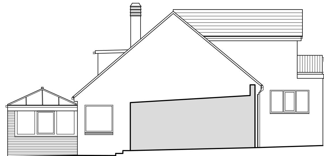
EXISTING SOUTH WEST ELEVATION
