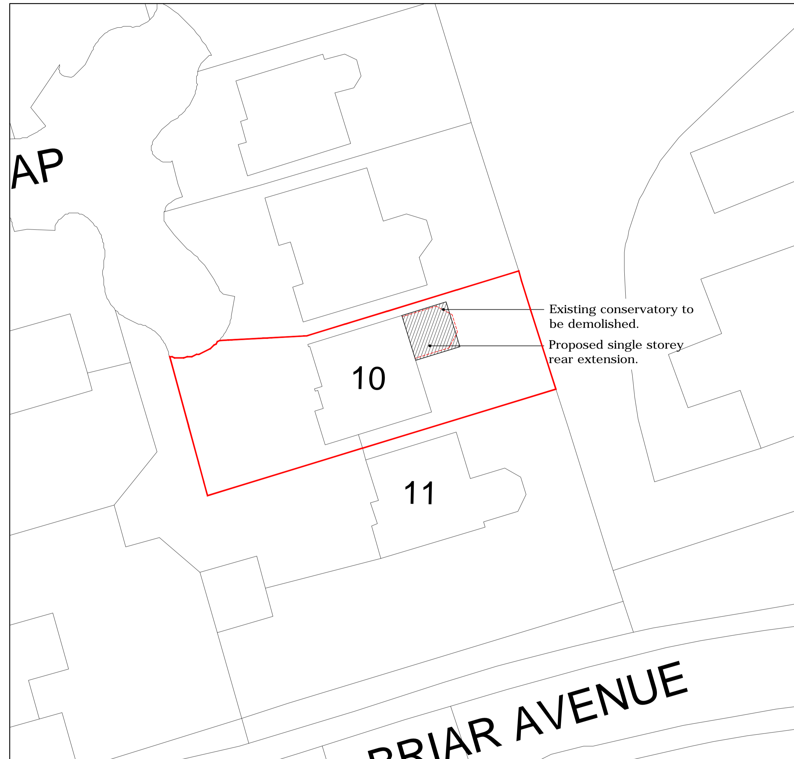
Block Plan (1:200)
