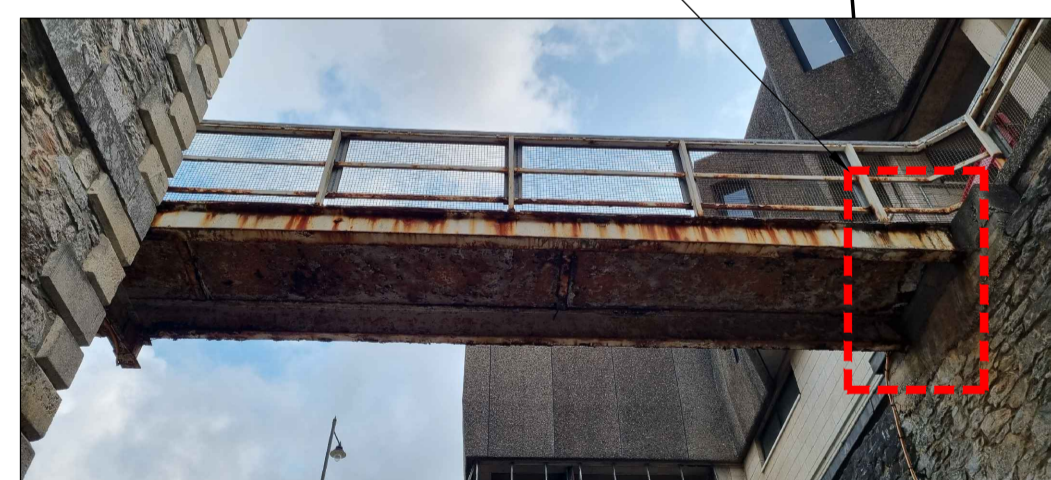
VIEW OF CORRODED STEEL WALKWAY ABOVE ROAD
