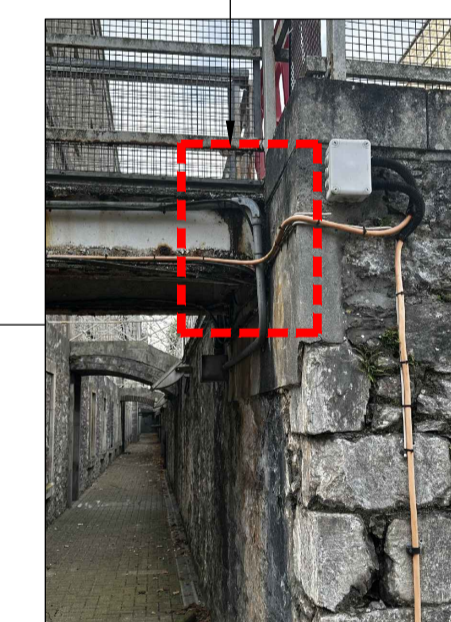
CONNECTION AT LOWER END OF GANTRY (NORTH WEST CORNER)
