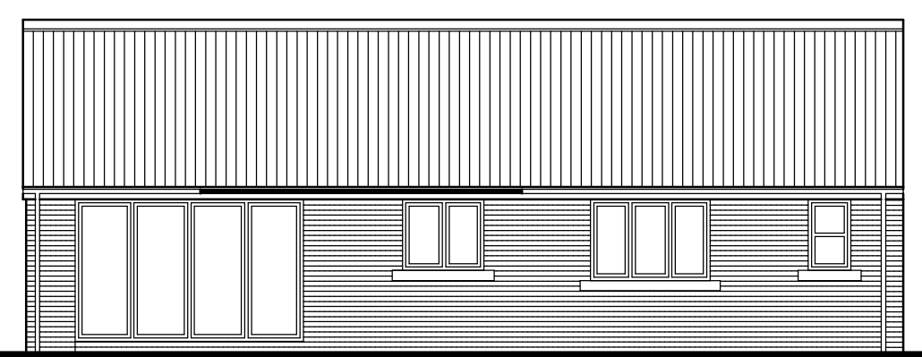
REAR ELEVATION
