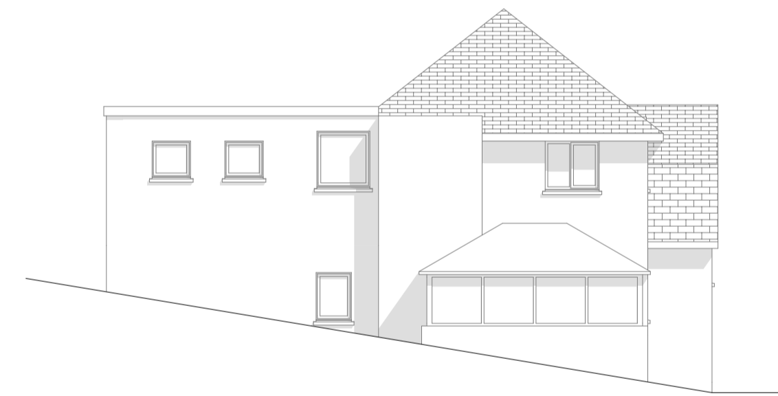
Existing Side Elevation Scale (A1): 1:100
