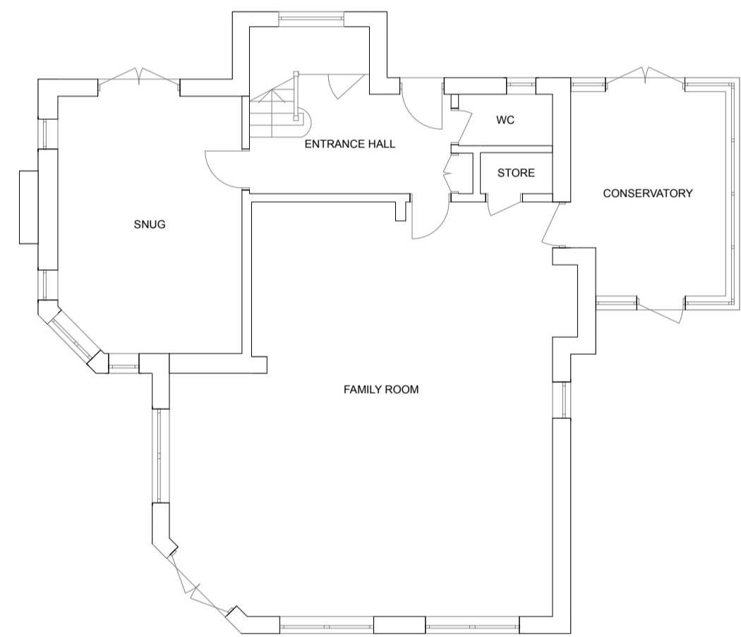
Existing Ground Floor Plan Scale (A1): 1:100
