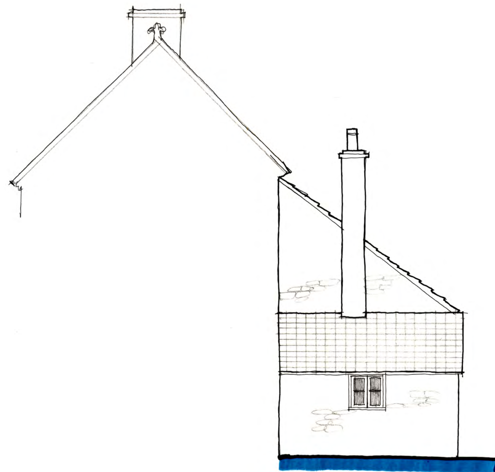
ELEVATIONS 1:50 SOUTH
