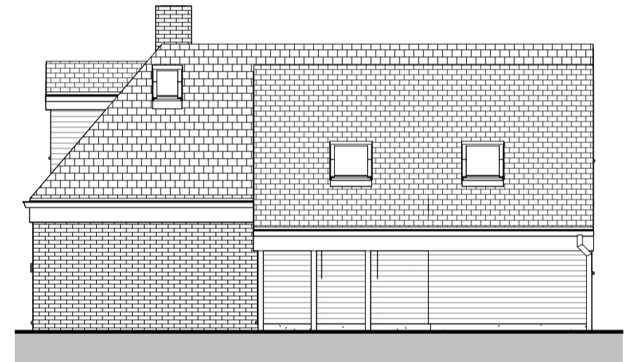
4 Existing West Elevation 1 : 100
