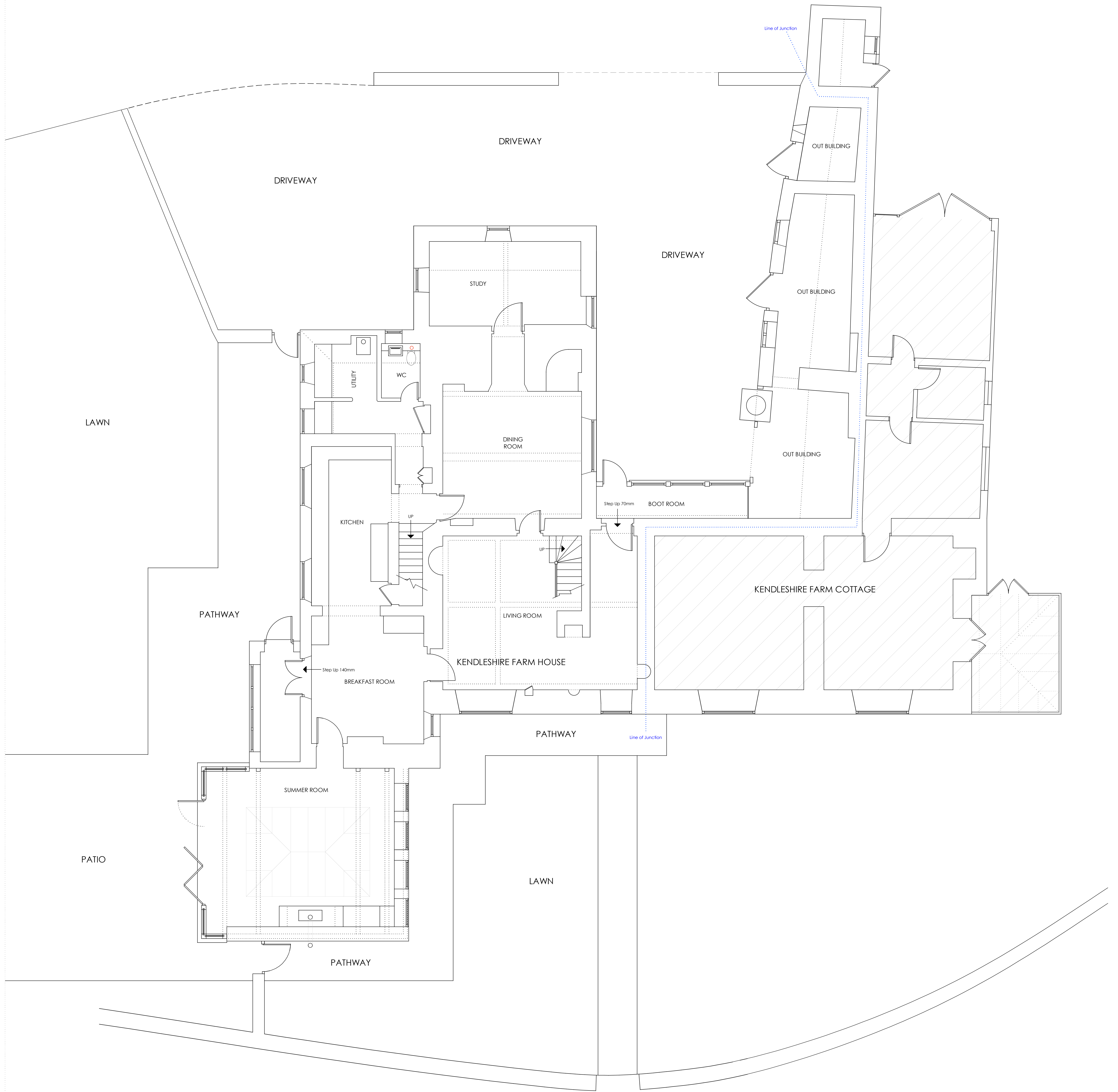
GROUND FLOOR PLAN SCALE 1:50
