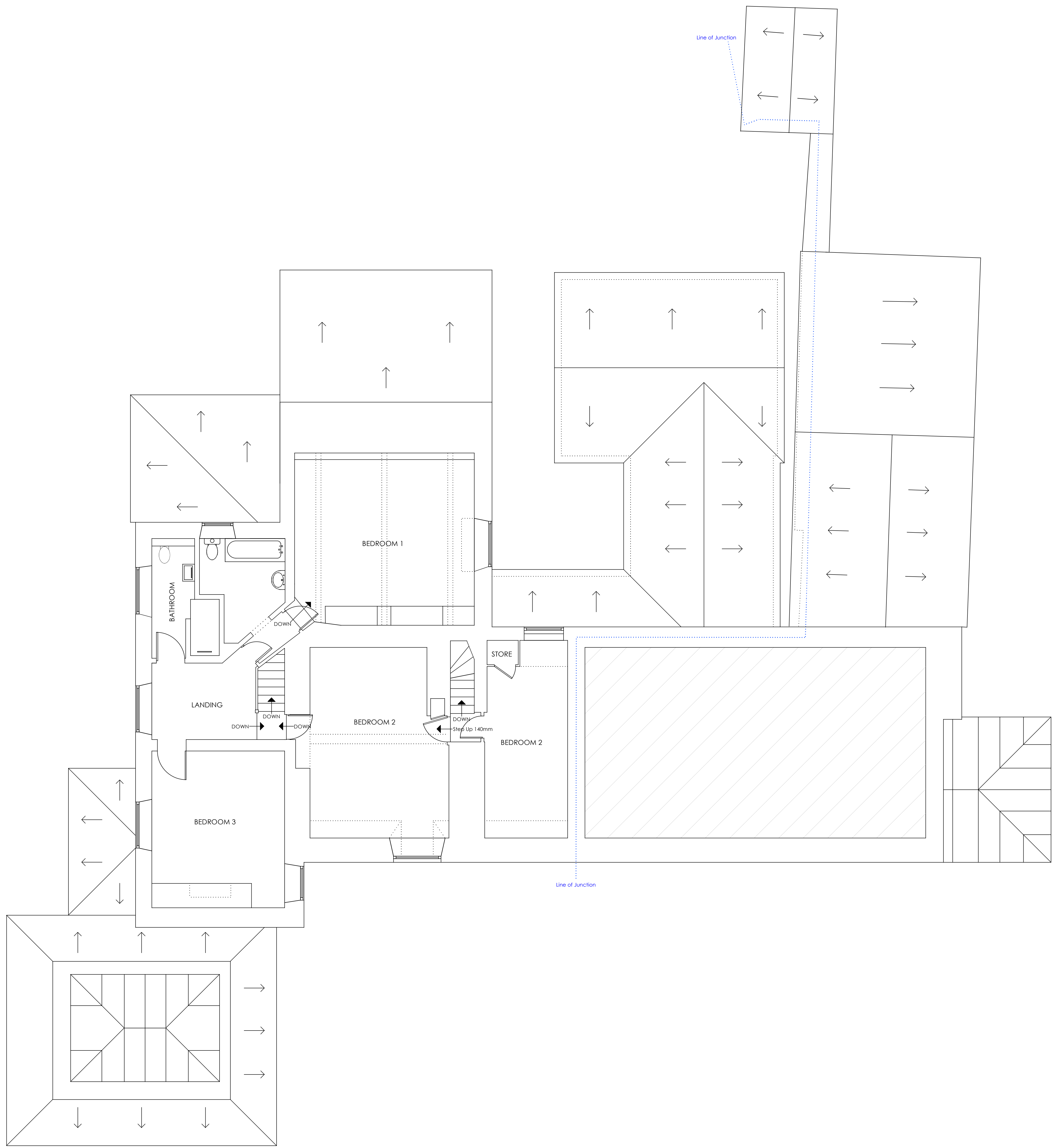
FIRST FLOOR PLAN SCALE 1:50
