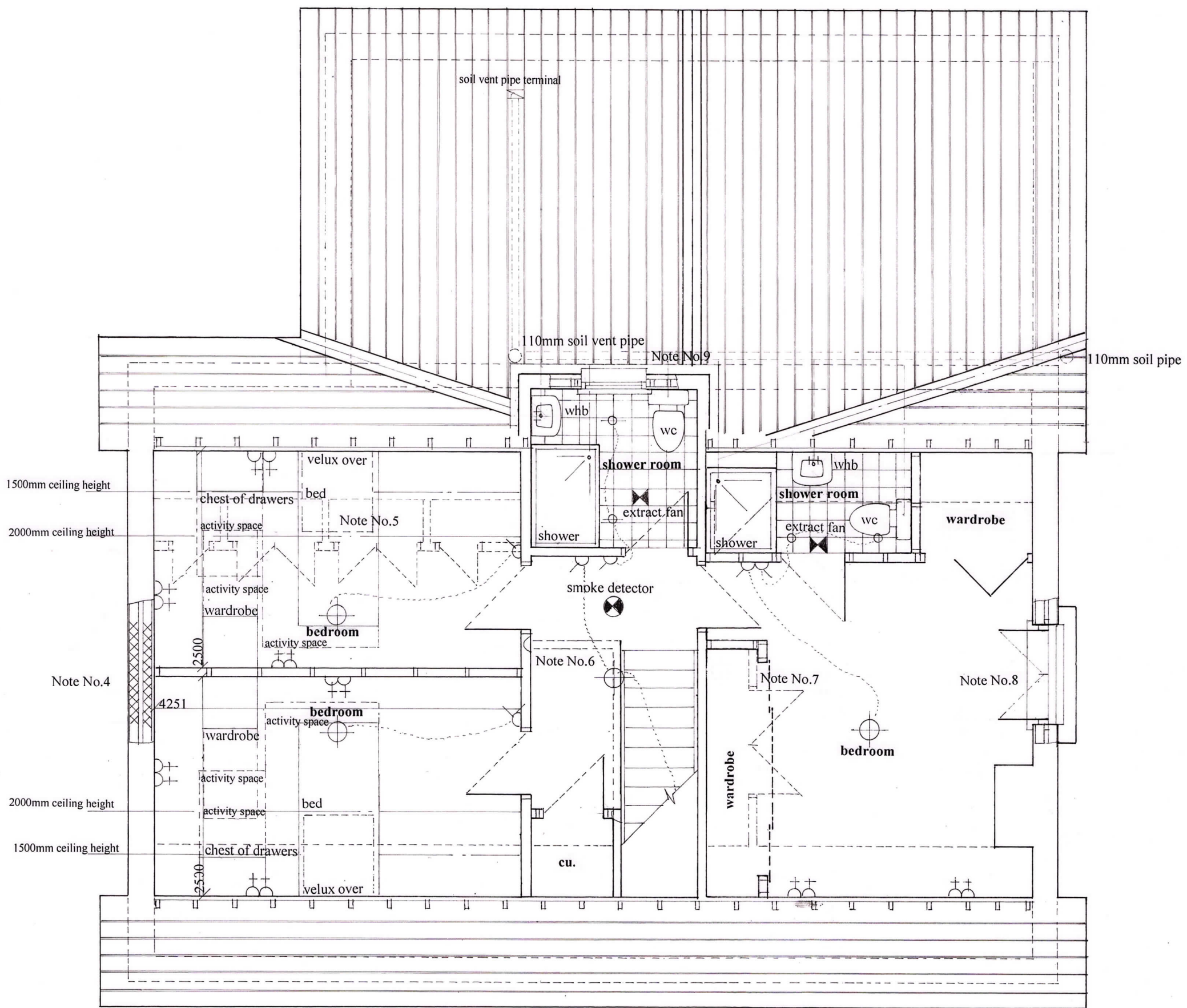
UPPER FLOOR PLAN as PROPOSED 1:50
