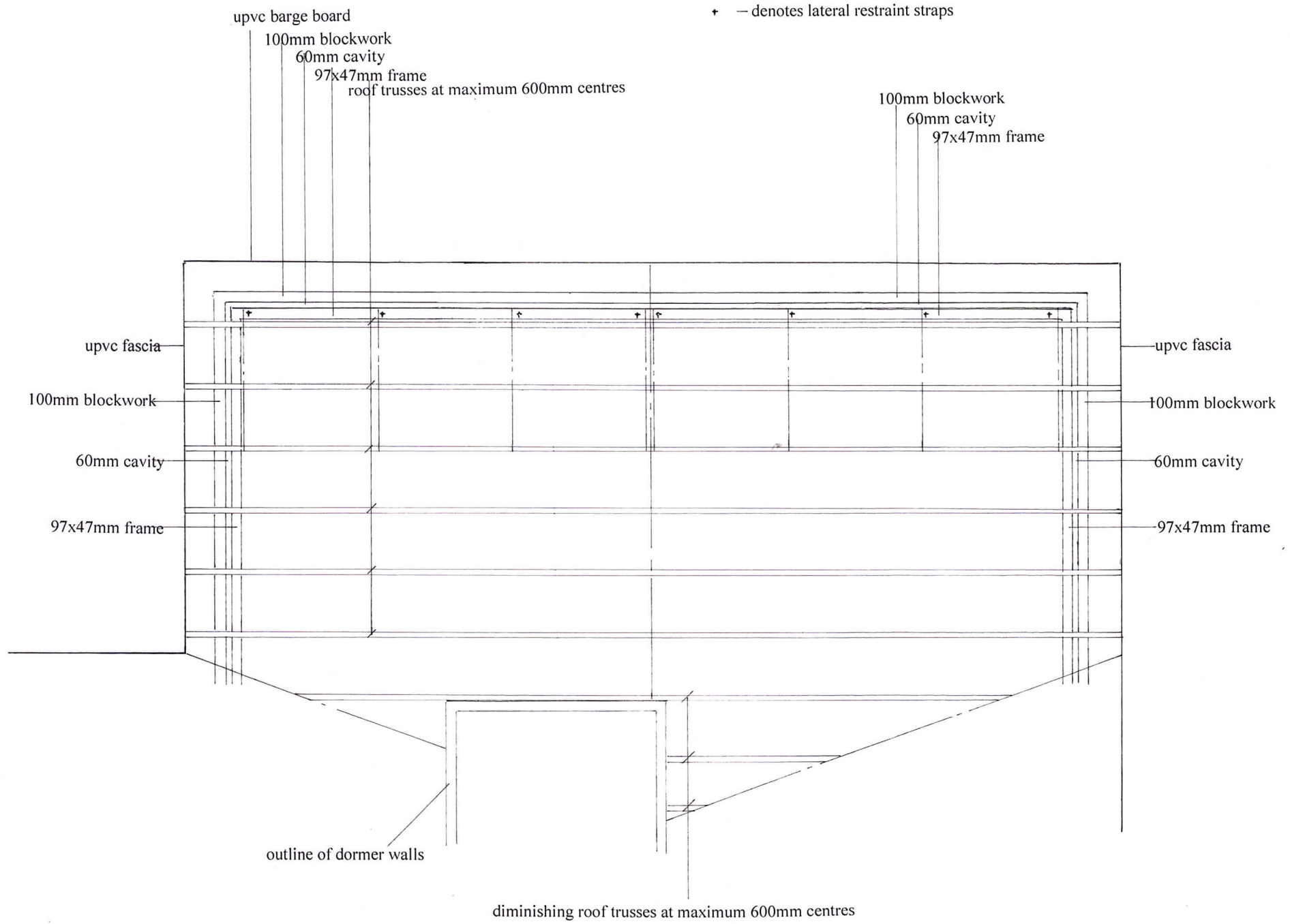
EXTENSION ROOF TRUSS LAYOUT PLAN 1:50
