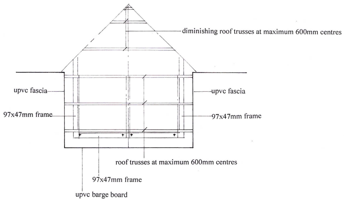
PORCH ROOF TRUSS LAYOUT PLAN 1:50
