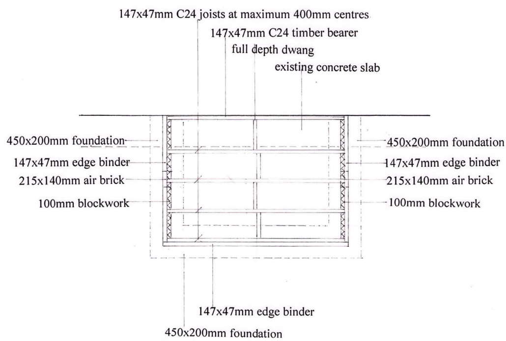
PORCH FOUNDATION/UNDERBUILDING LAYOUT PLAN 1:50
