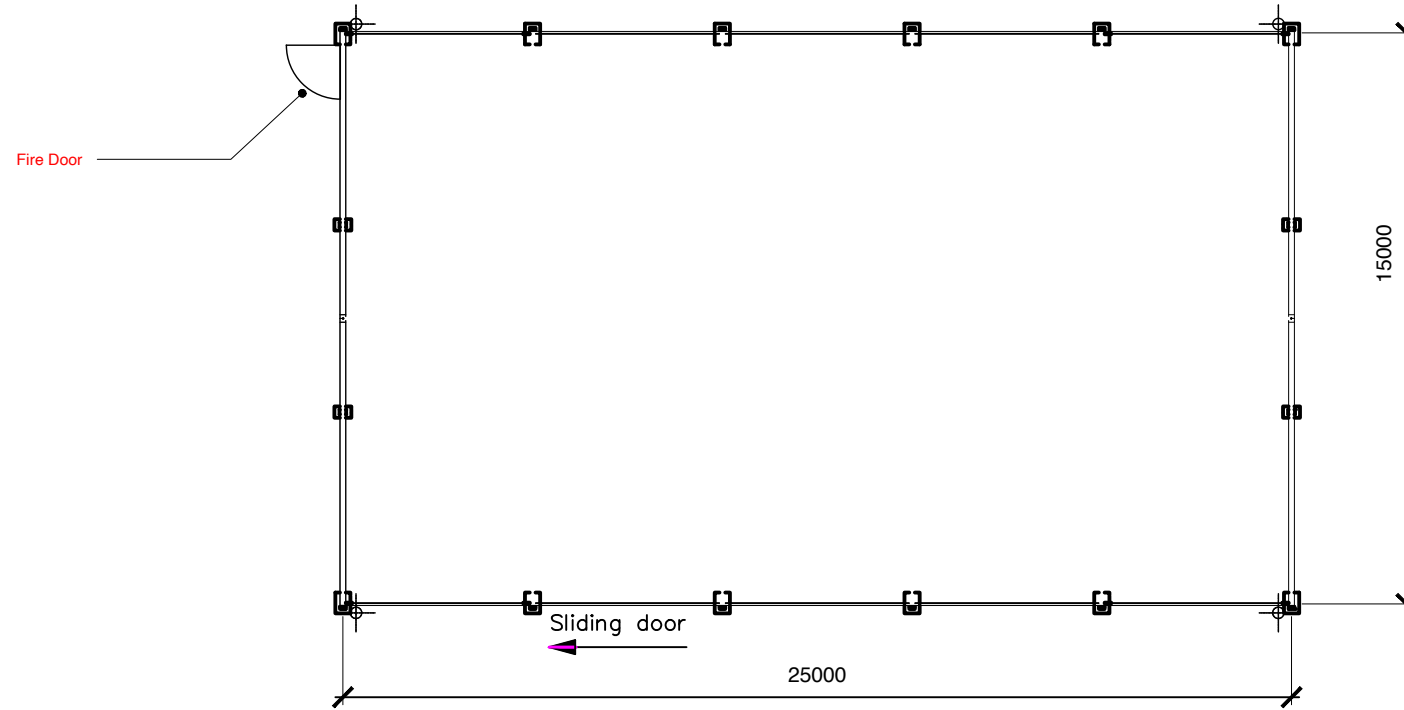
Proposed Floor Plan Scale 1:200 @ A3
