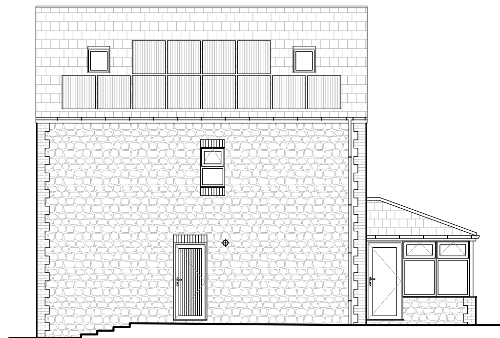
REAR ELEVATION 1:100
