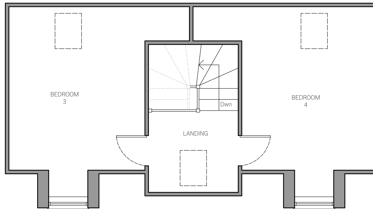
LOFT FLOOR PLAN 1:50
