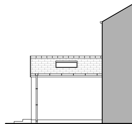
PROPOSED NORTH ELEVATION 1:100
