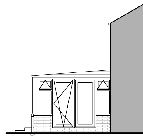
EXISTING NORTH ELEVATION 1:100
