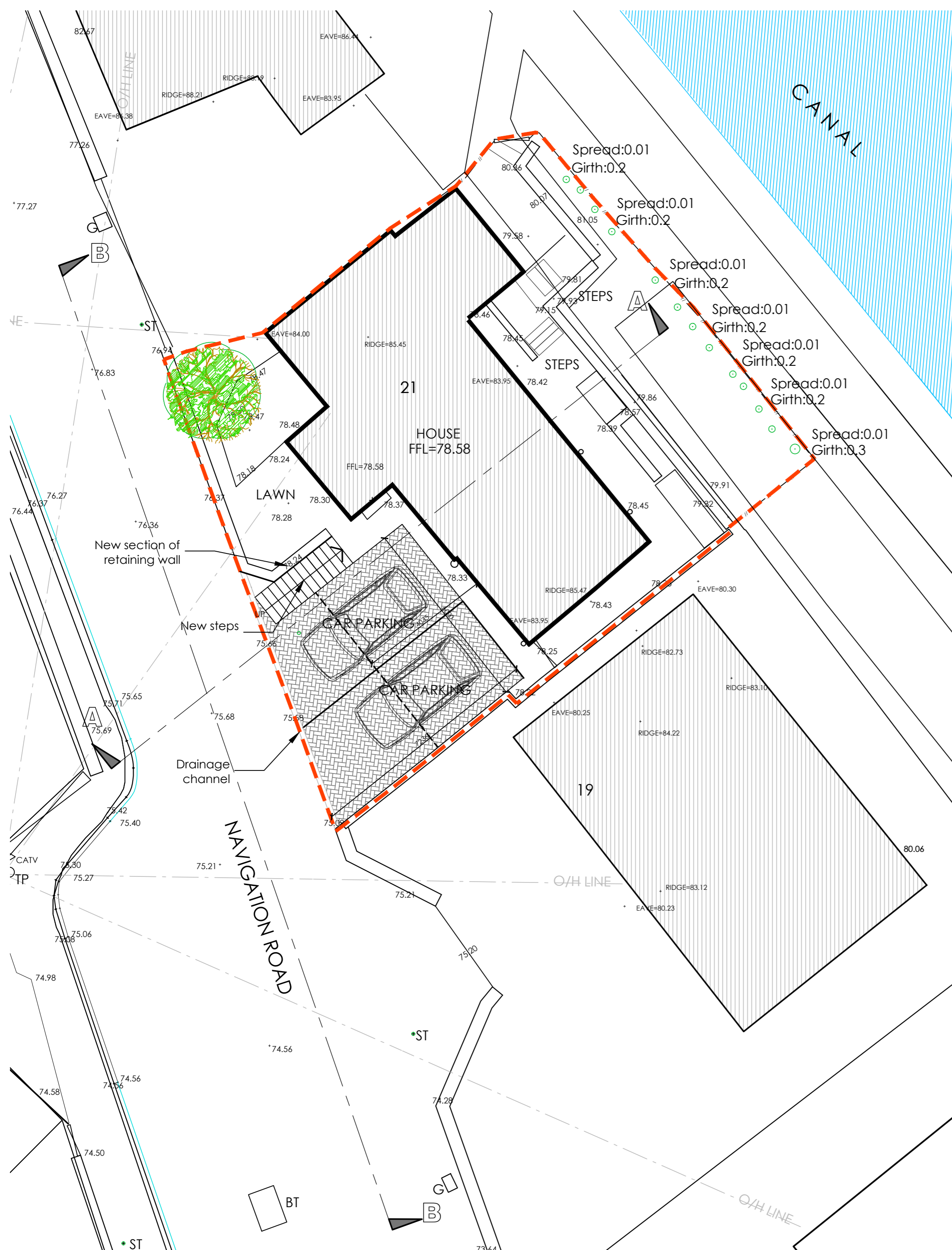
PLAN AS LOWER LEVEL (STREET LEVEL)
