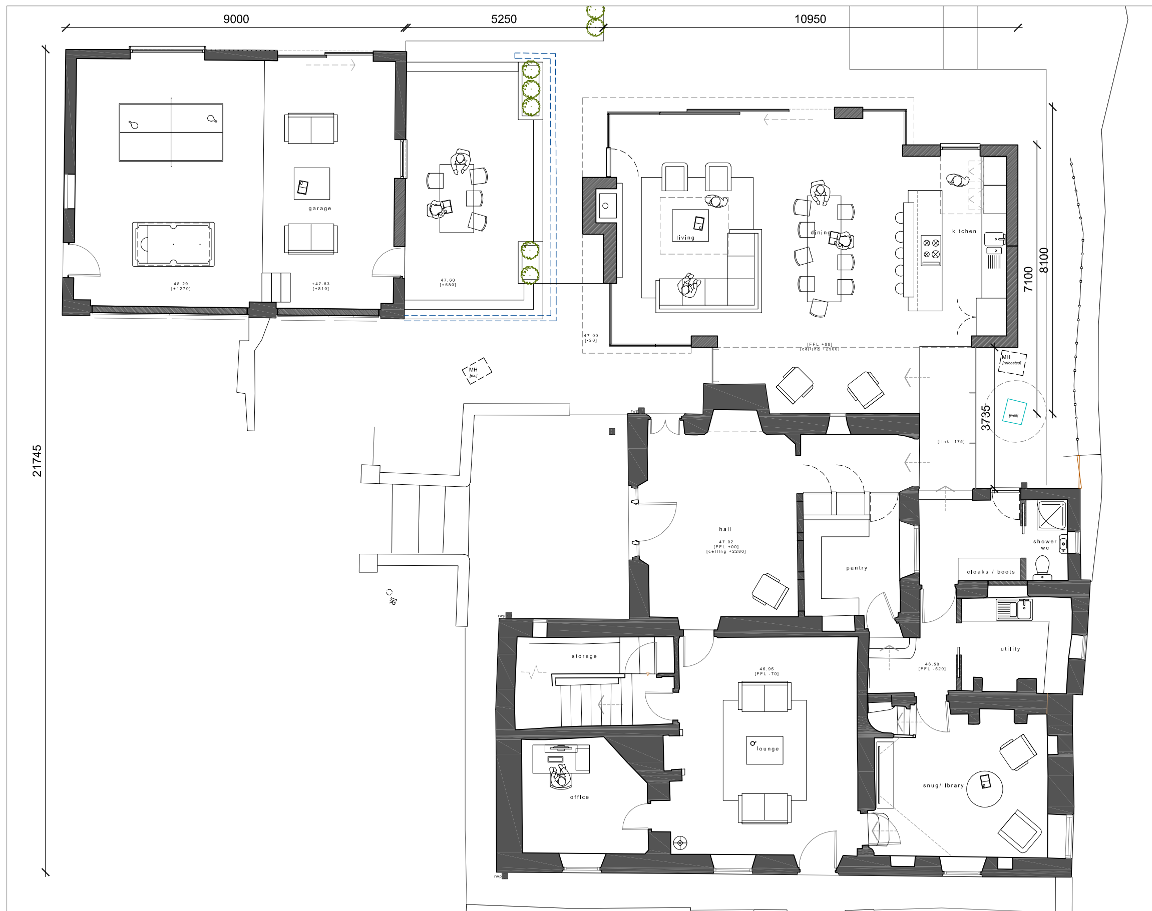
- Ground Floor Layout Plan
