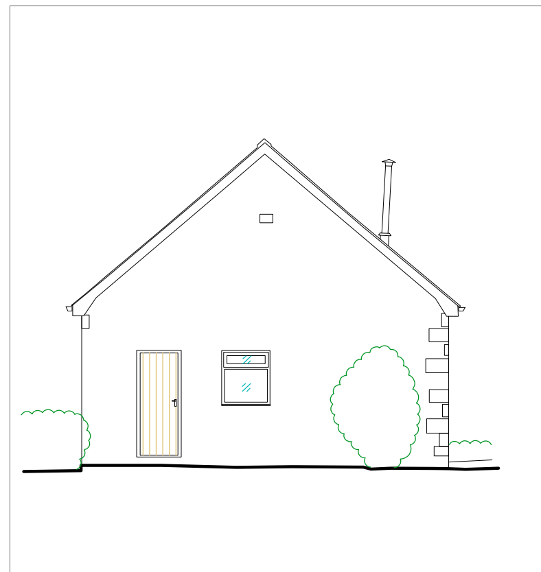
04 - Elevation to side / North
