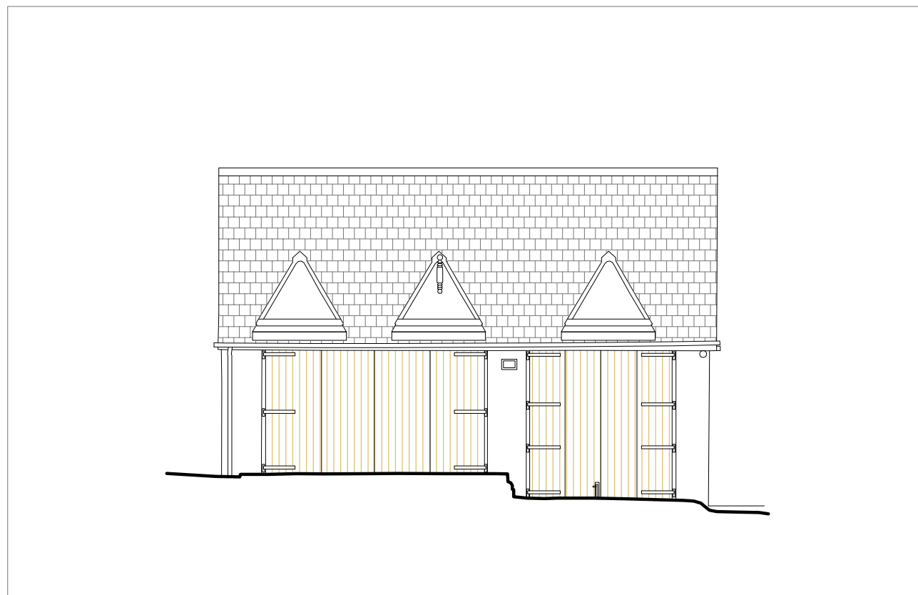
01 - Elevation to front / East
