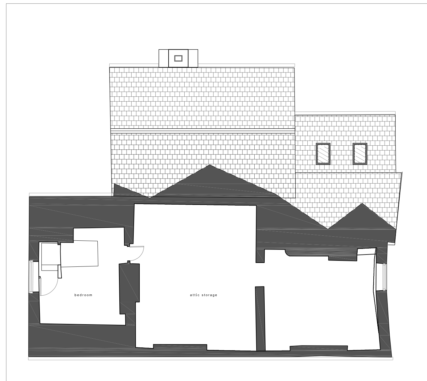
- Second Floor Layout Plan
