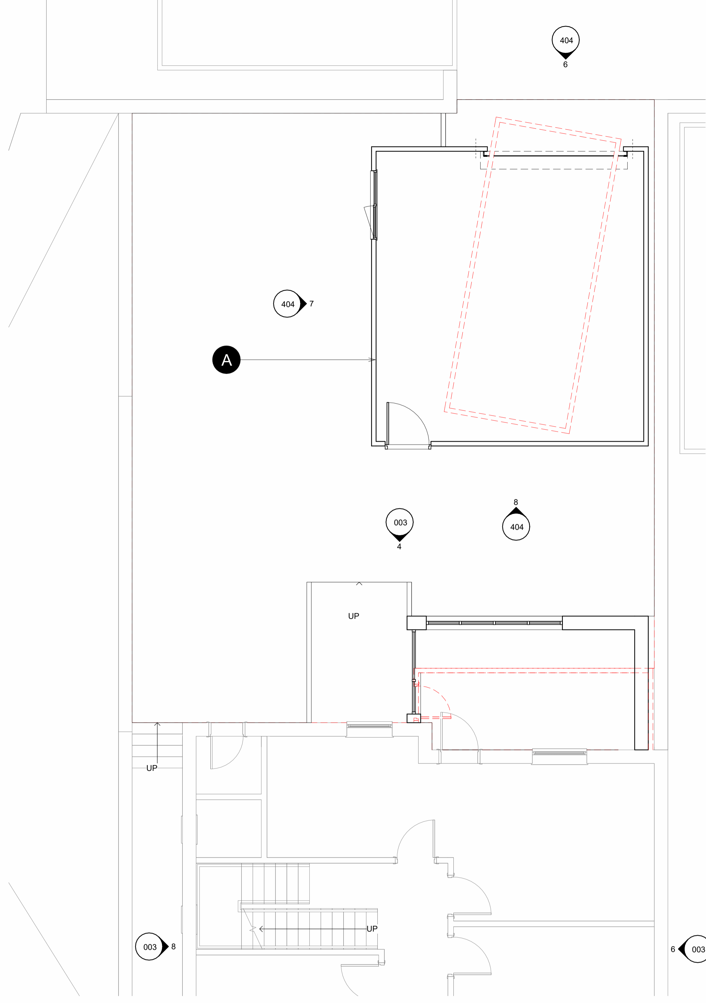
3 Plan of Proposed New Garage SCALE: 1 : 50
