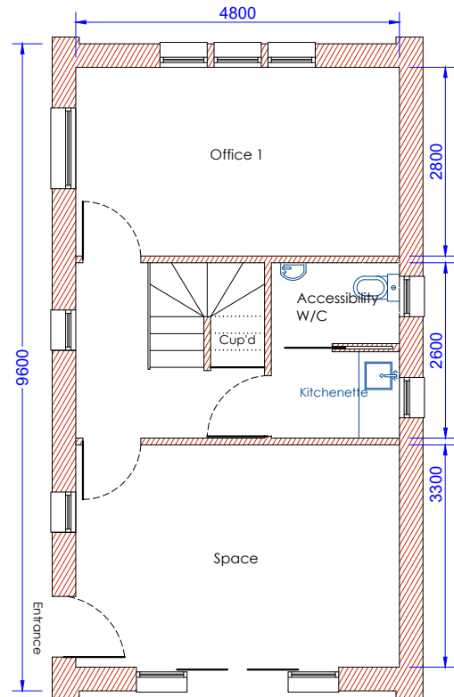
Office Unit Ground Floor
