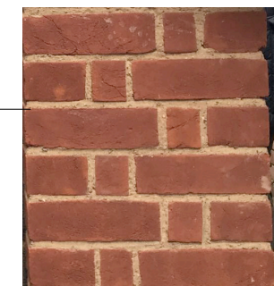
Soft brick laid in lime mortar
