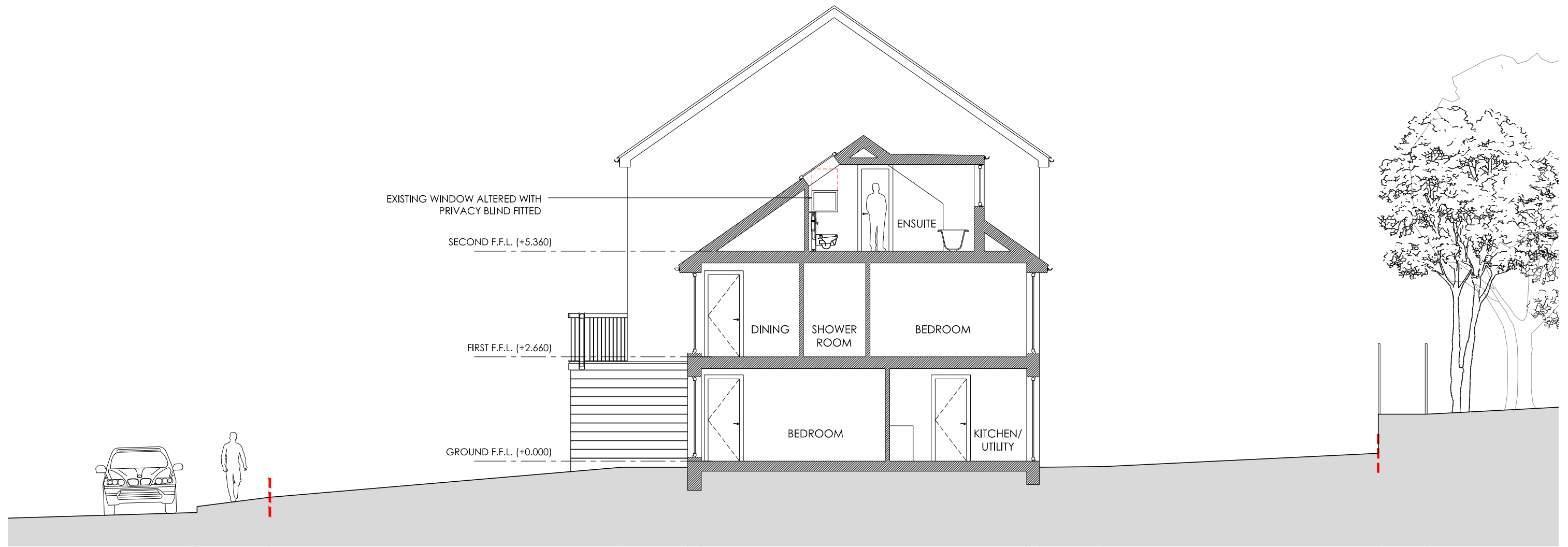
PROPOSED SECTION C
