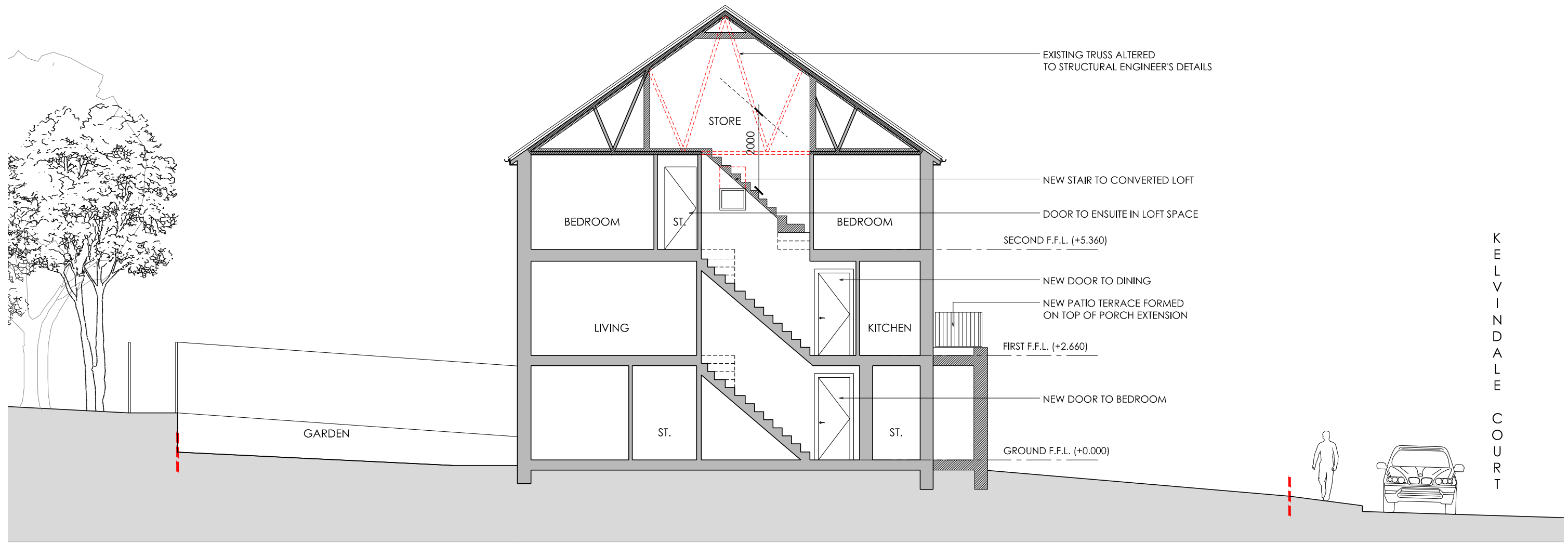
PROPOSED SECTION B
