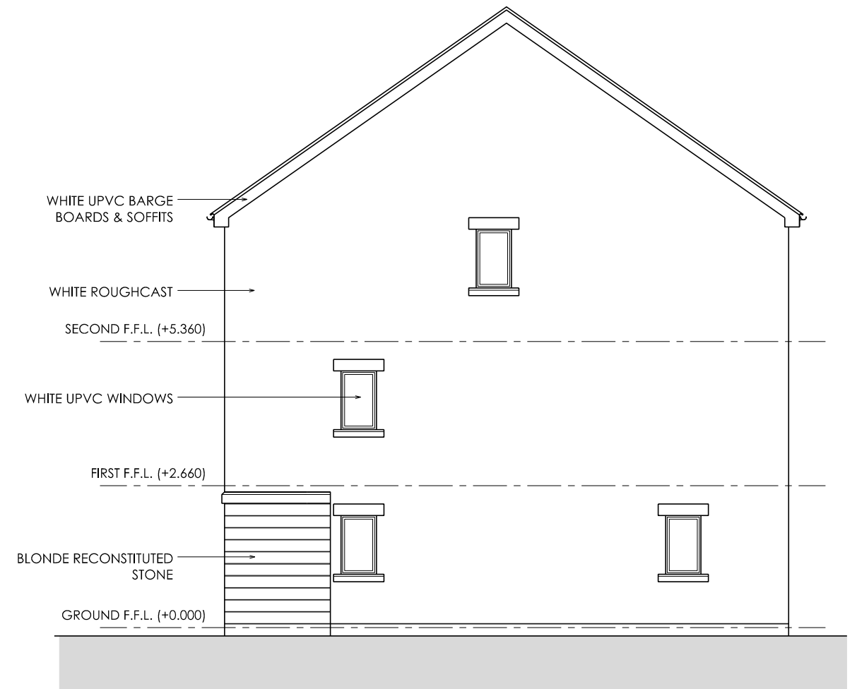
EXISTING NORTH ELEVATION
