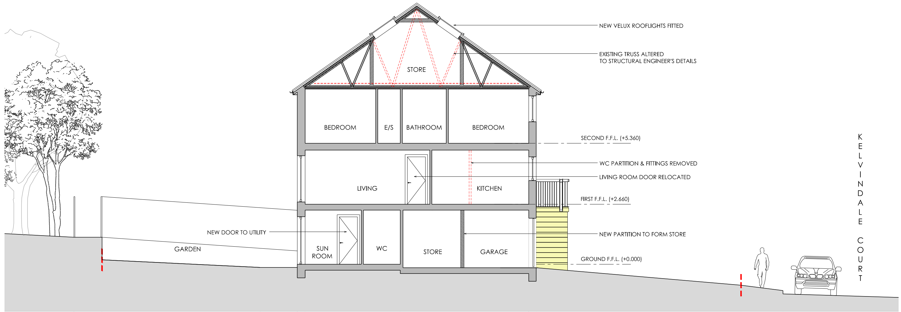
PROPOSED SECTION A
