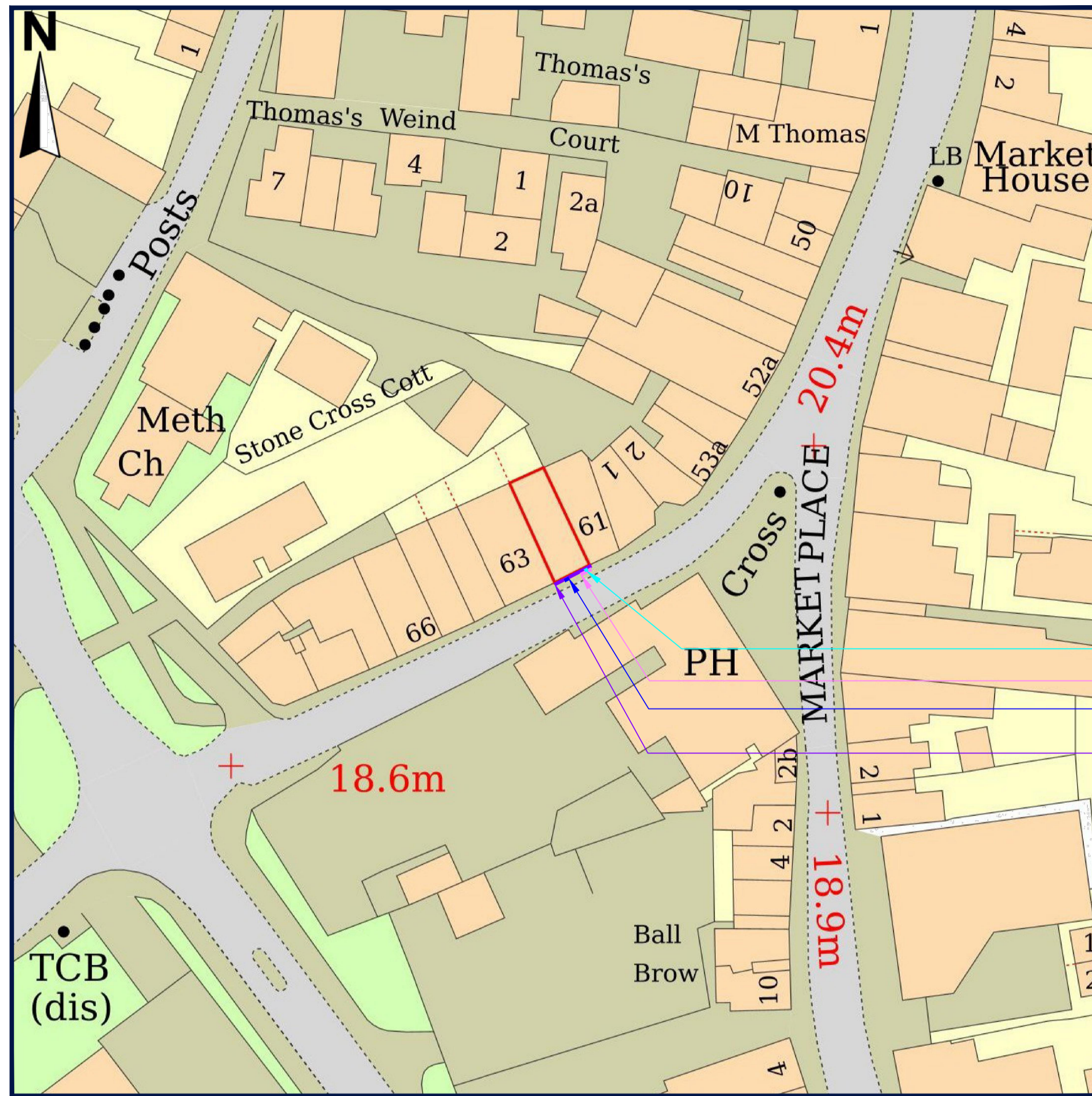
BLOCK PLAN - 1:500
