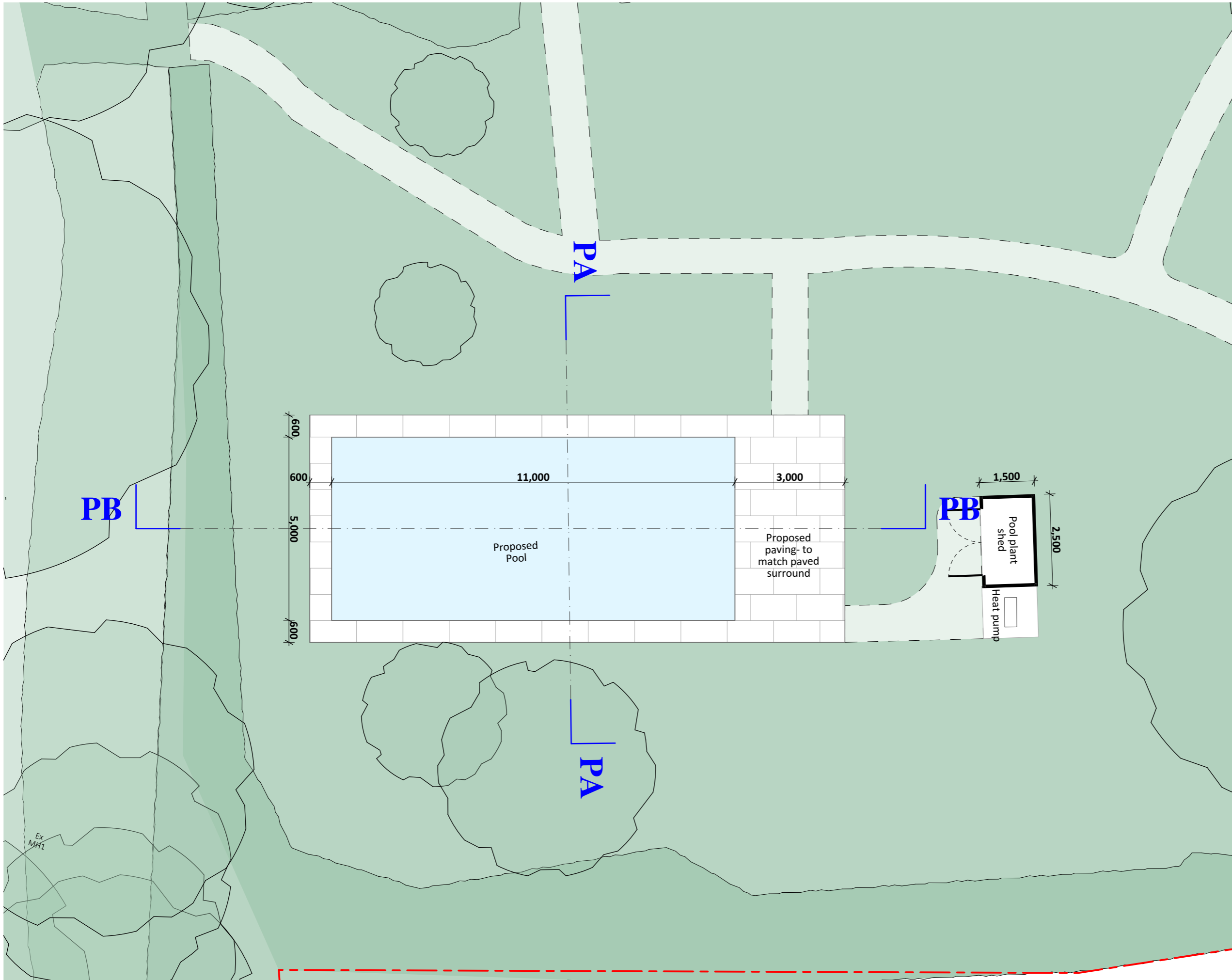
Proposed Swimming Pool Plan 1:100
