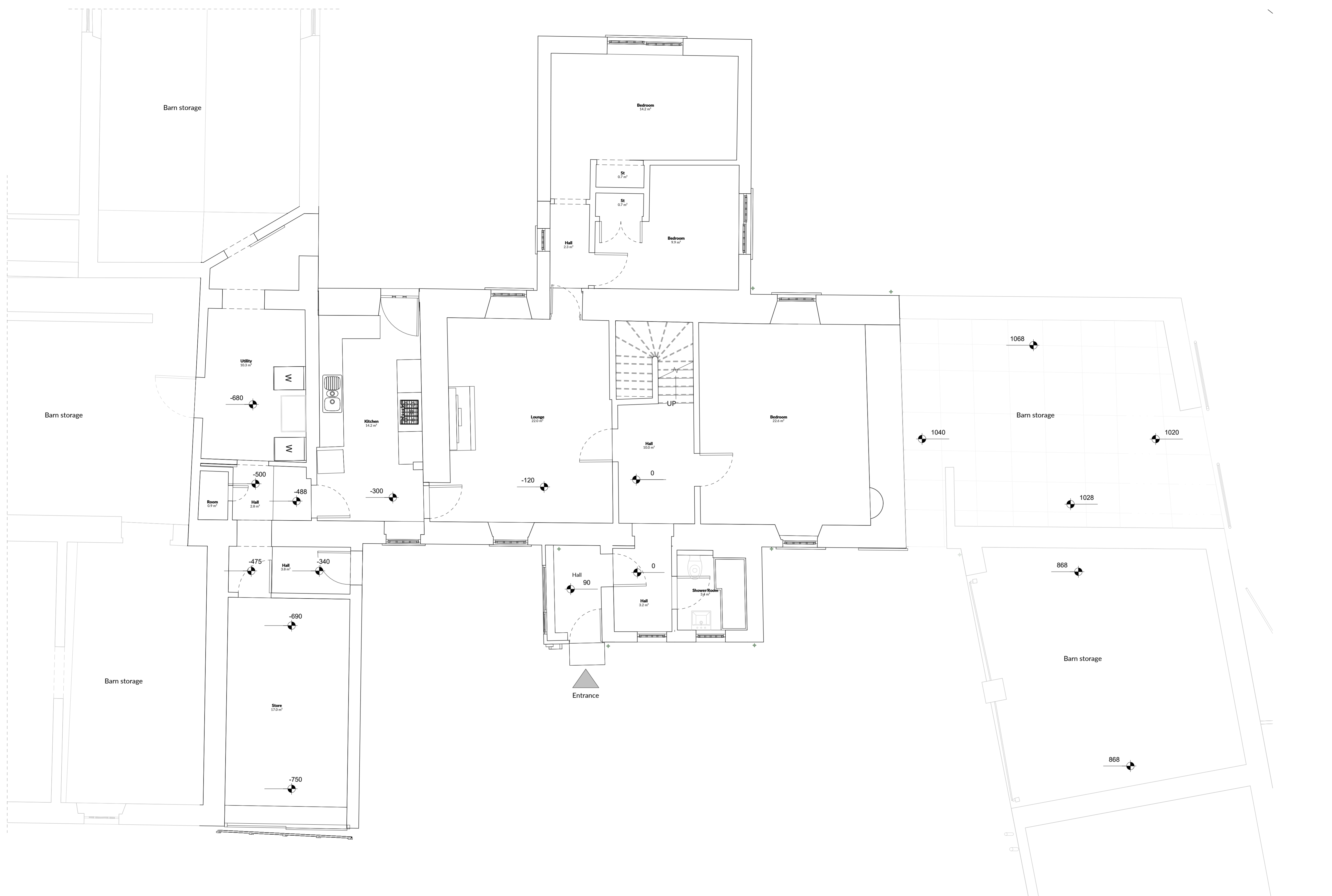
00.0 Existing Ground Floor Plan
