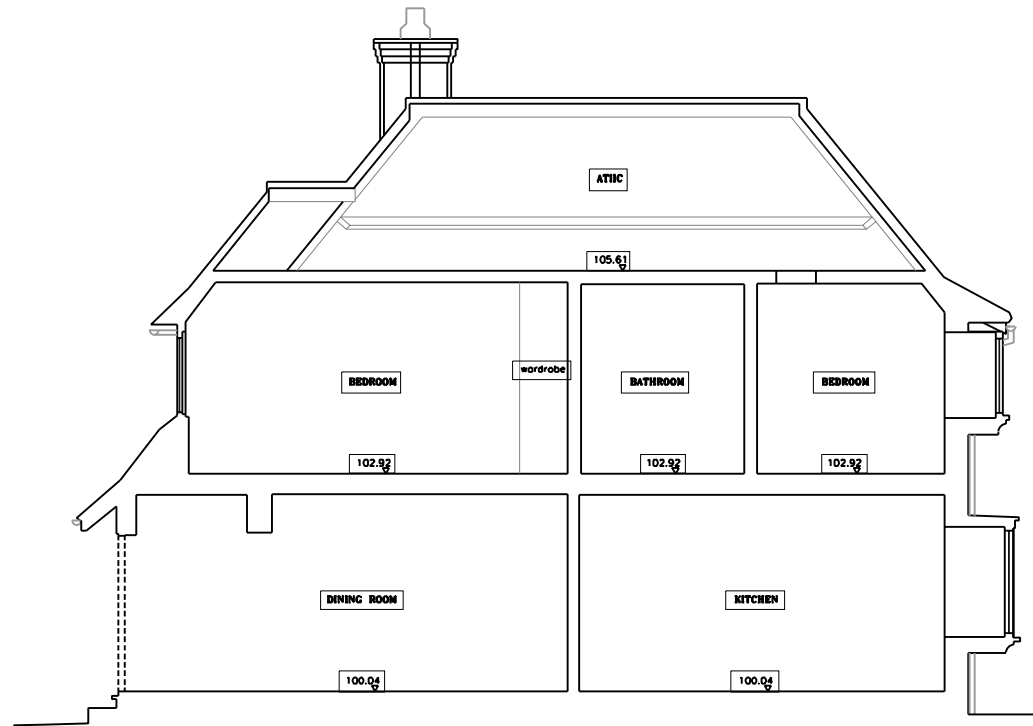
EXISTING SECTION
