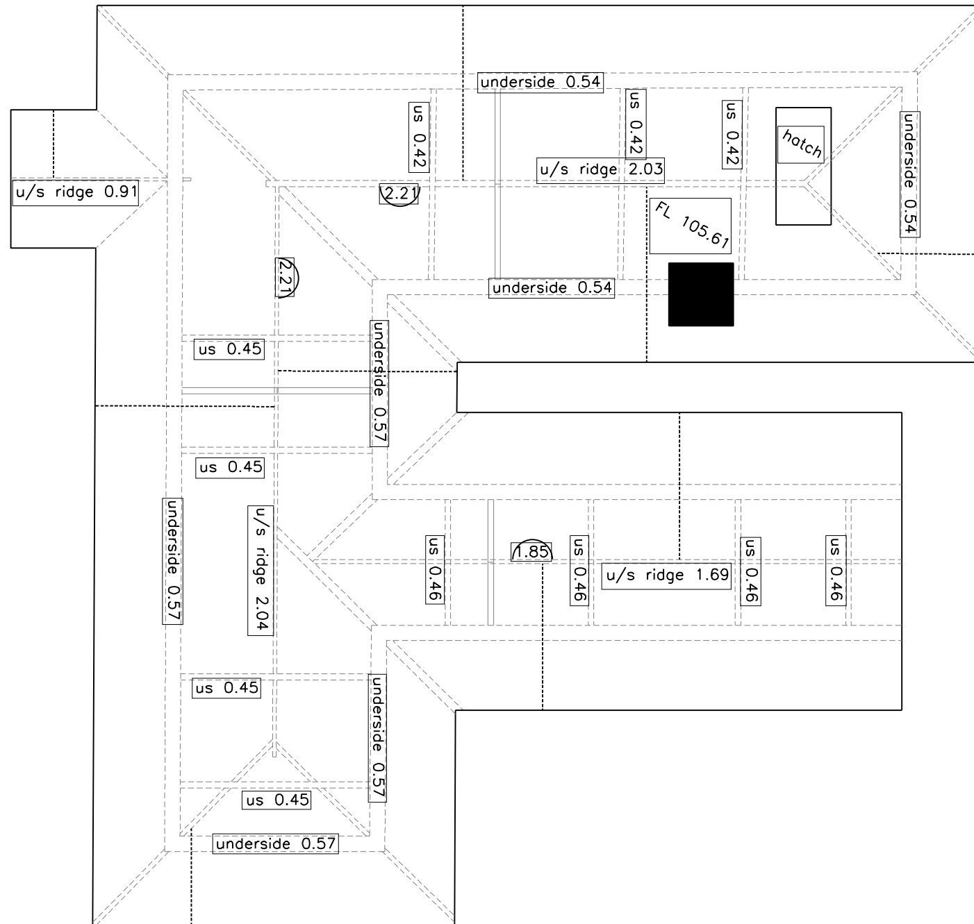
EXISTING ATTIC LAYOUT
