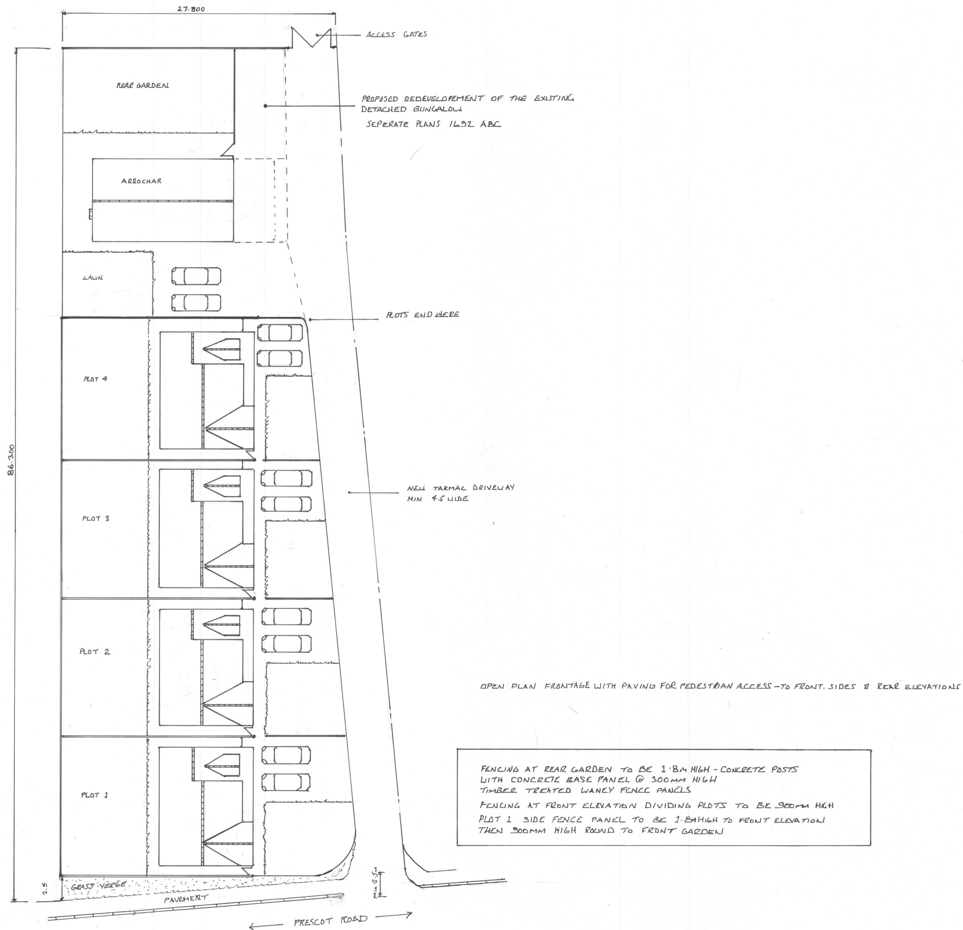
PROPOSED SITE BLOCK PLAN
