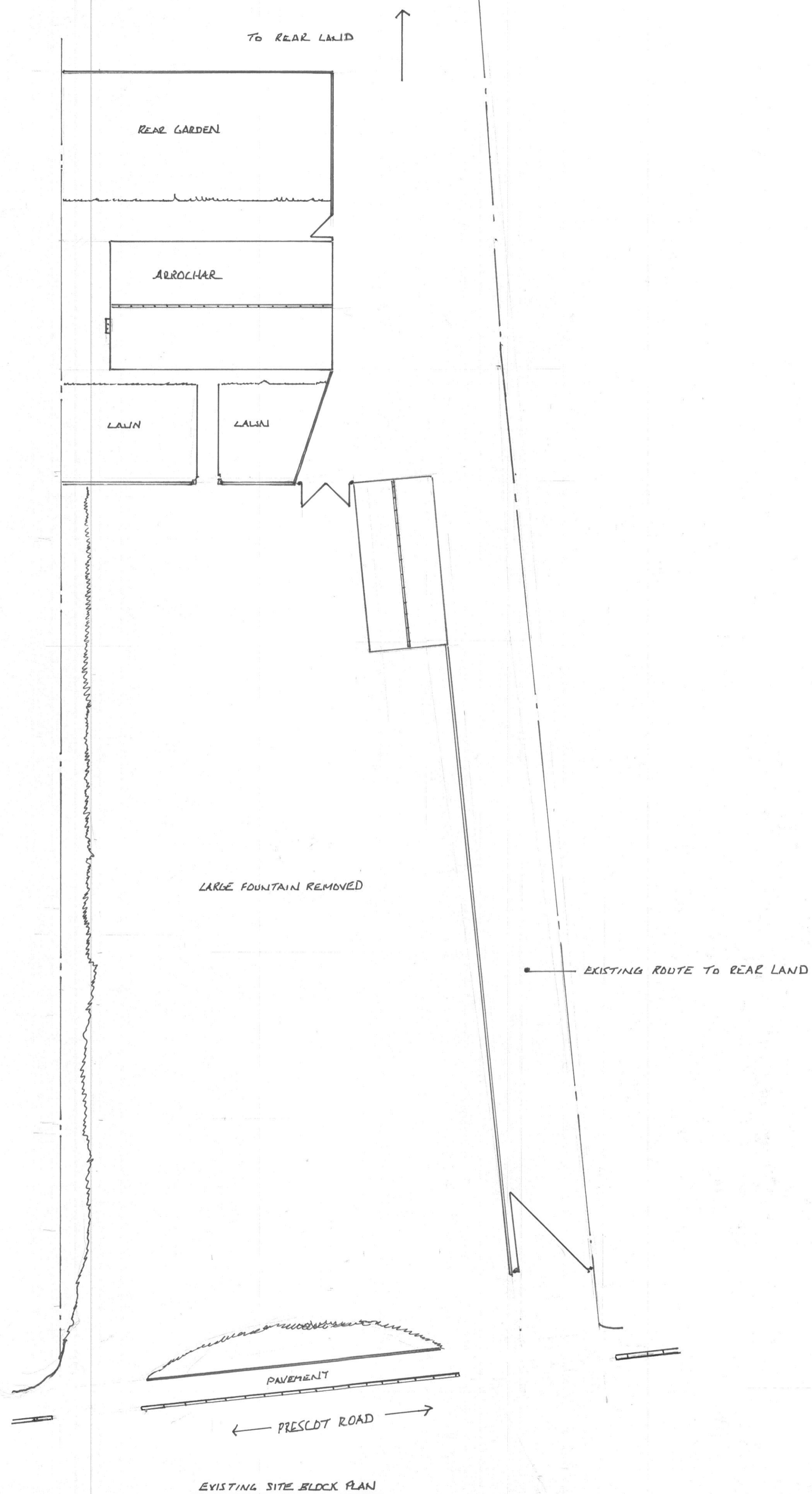
EXISTING SITE BLOCK PLAN
