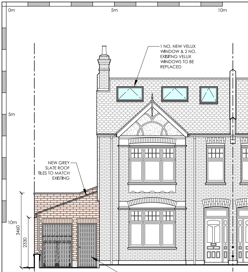
1 - FRONT ELEVATION
