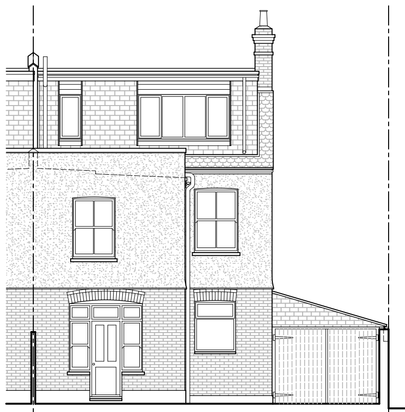
3 - REAR ELEVATION
