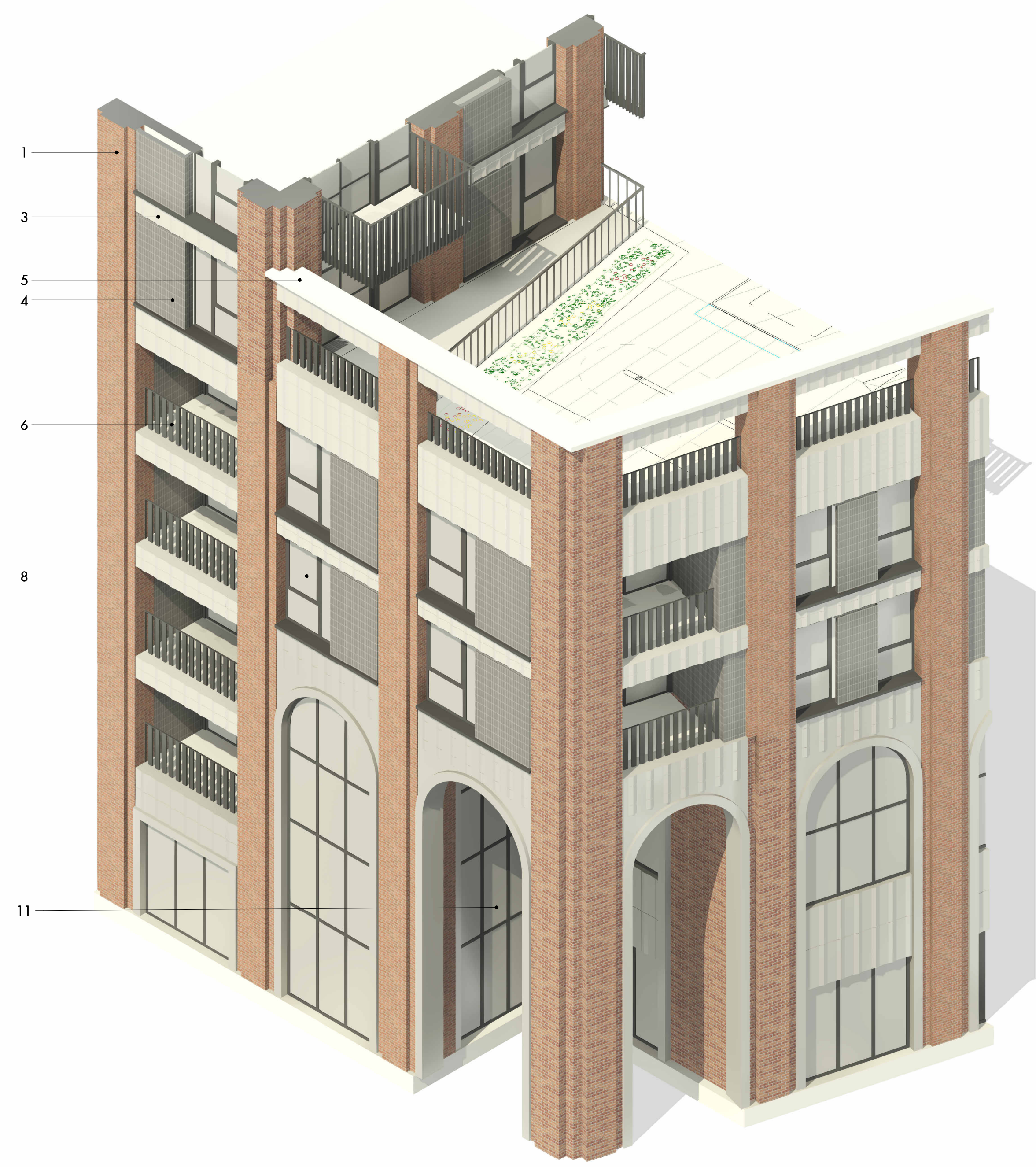
2 07_Bay Study 01 - Entrance and Collonade
