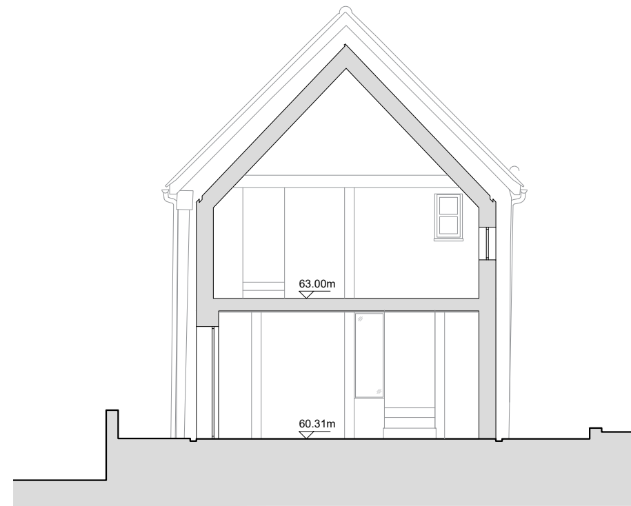
02 | PROPOSED SECTION D-D
