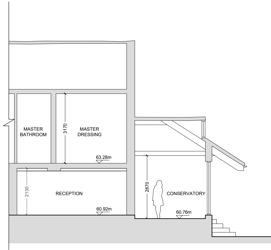
01 | EXISTING SECTION A-A
