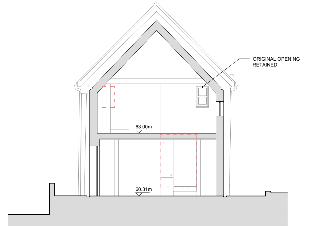
02 | PROPOSED SECTION D-D - DEMOLITION
