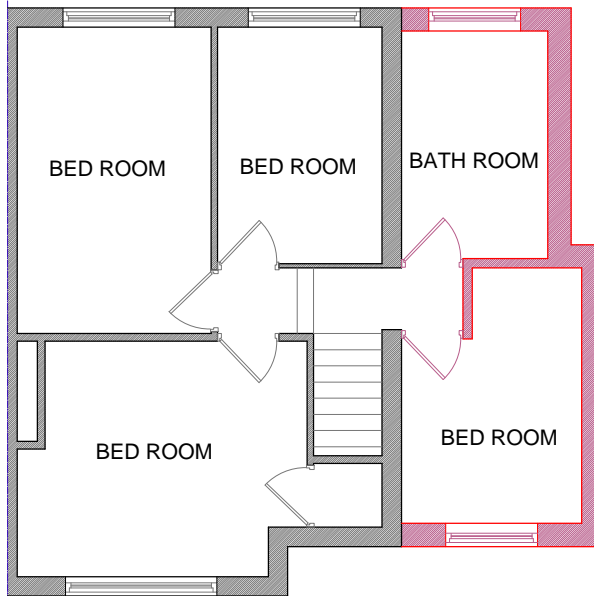
PROPOSED FIRST FLOOR PLAN Scale 1:100
