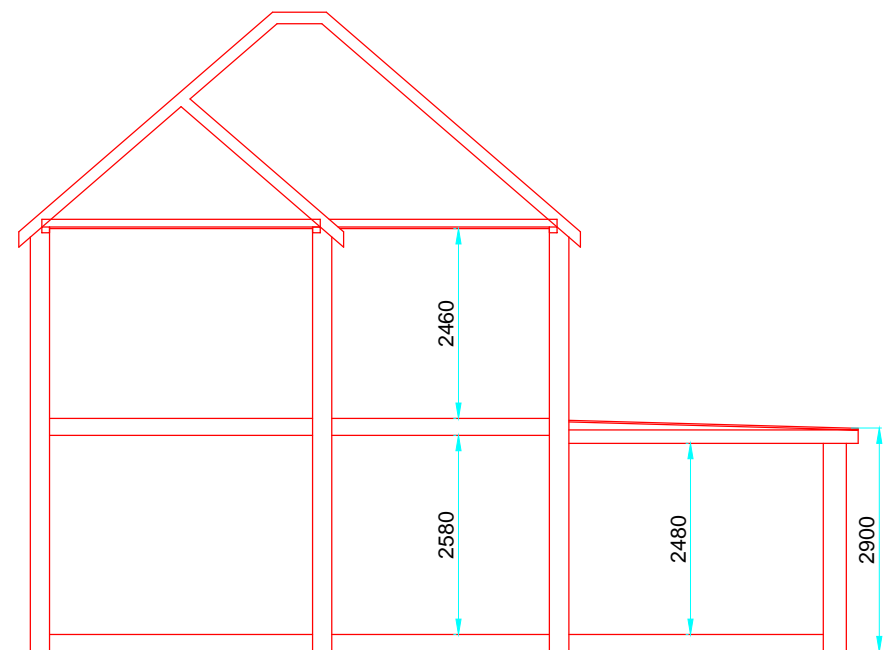
PROPOSED SECTION Scale 1:100
