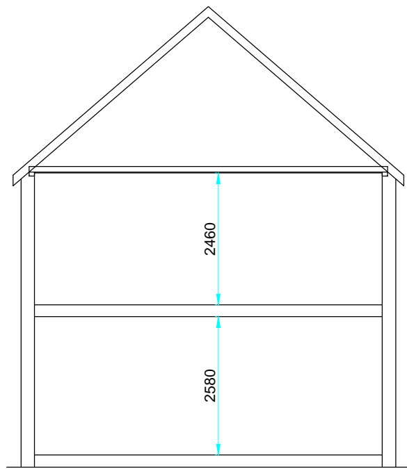
EXISTING SECTION Scale 1:100
