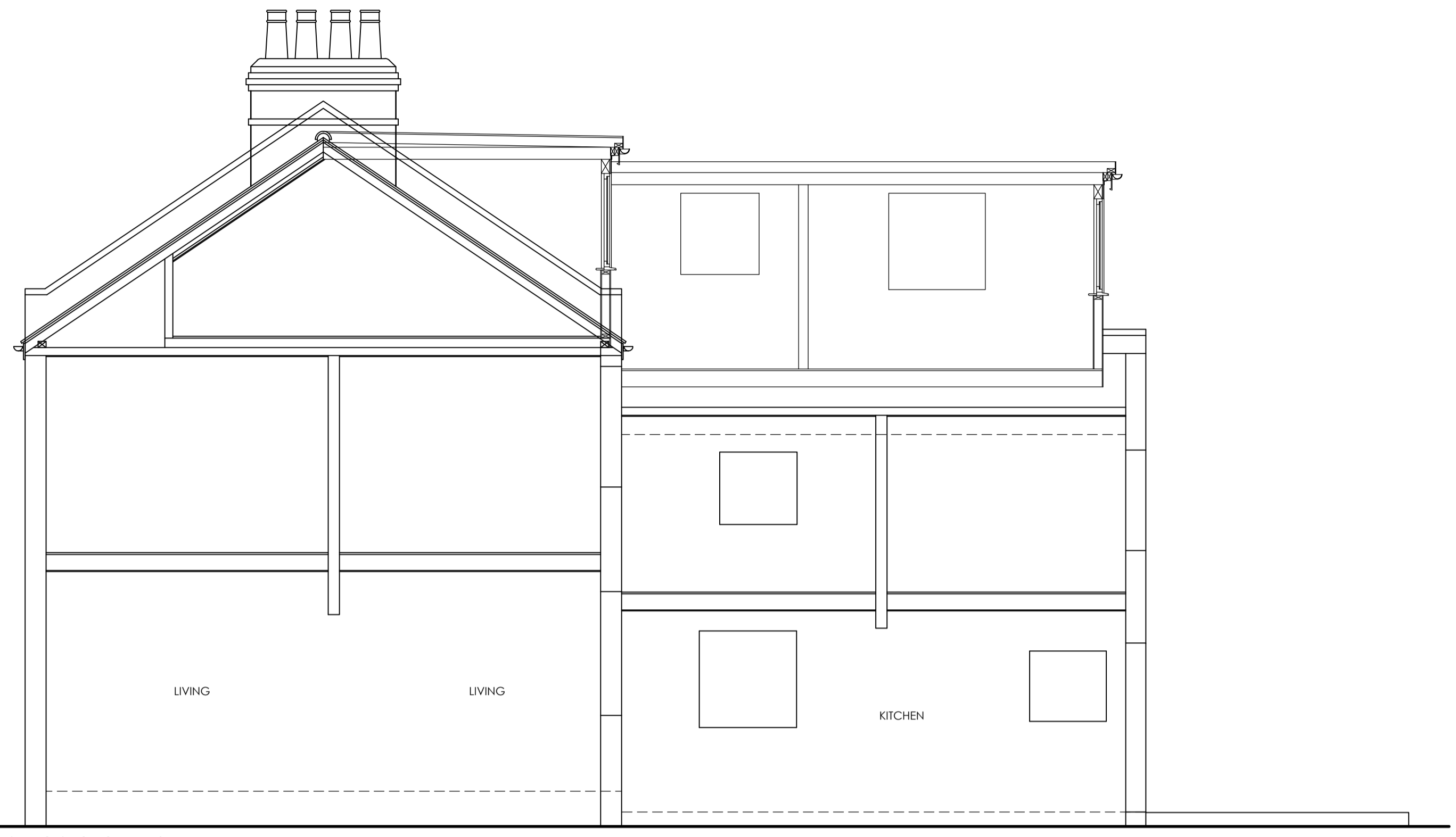
EXISTING SECTION 1:50
