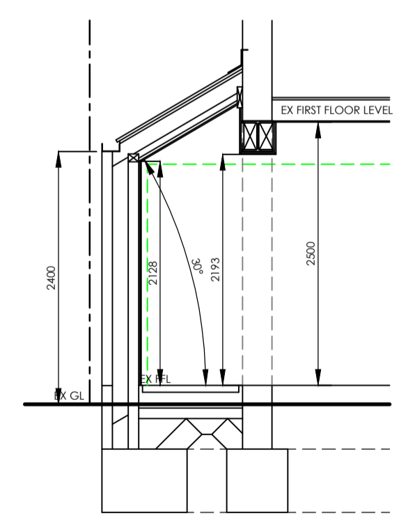
PROPOSED SECTION 1:50
