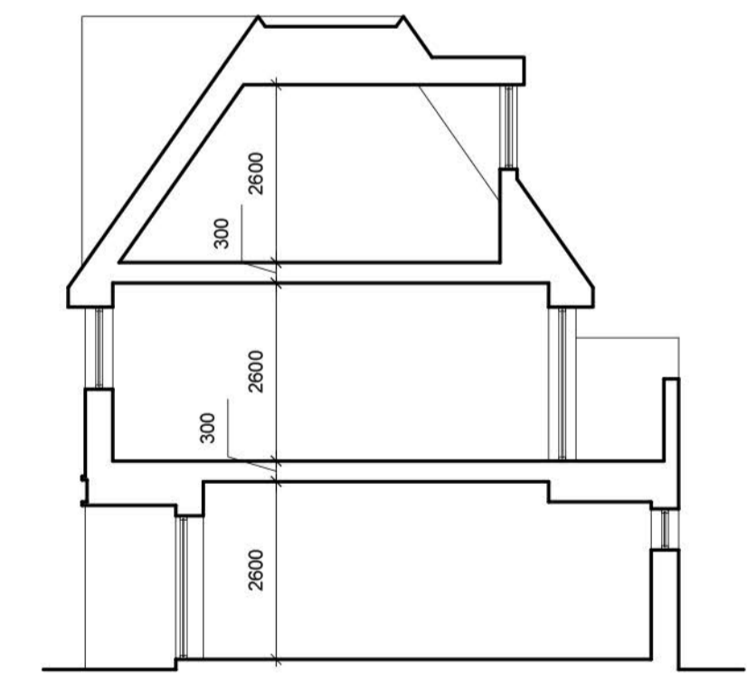
Proposed Section Looking West 1:100
